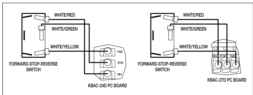
FIGURE 3 - CONNECTION DIAGRAM
