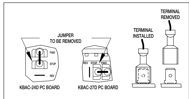
FIGURE 2 - JUMPER ASSEMBLY
