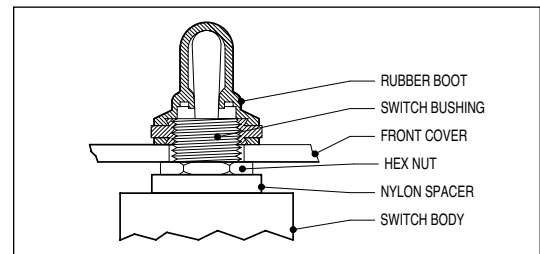
FIGURE 1 - MOUNTING THE SWITCH
