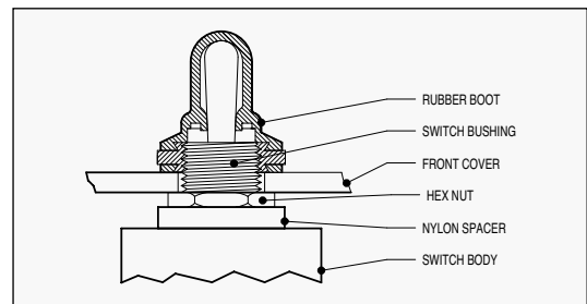
FIGURE 1 – MOUNTING THE POWER ON/OFF SWITCH
