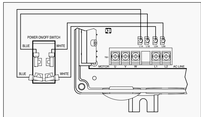
FIGURE 3 – CONNECTION DIAGRAM
