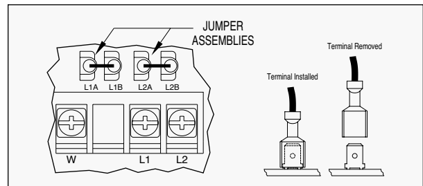
FIGURE 2 – JUMPER ASSEMBLIES
